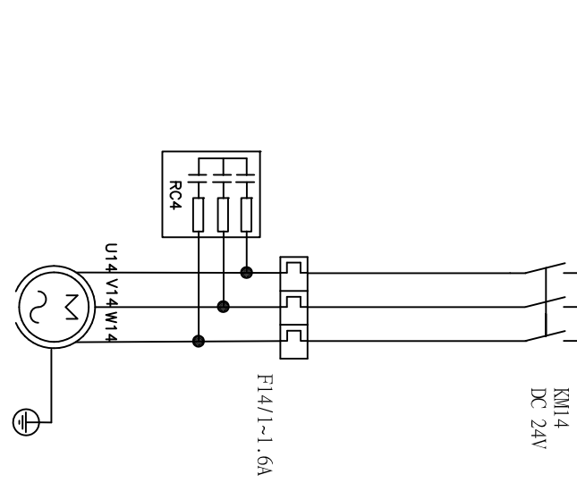
CHAIN MOTOR
